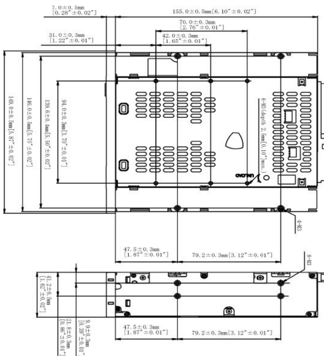
Figure 2-2b: SDX-500C/R Mounting Holes
