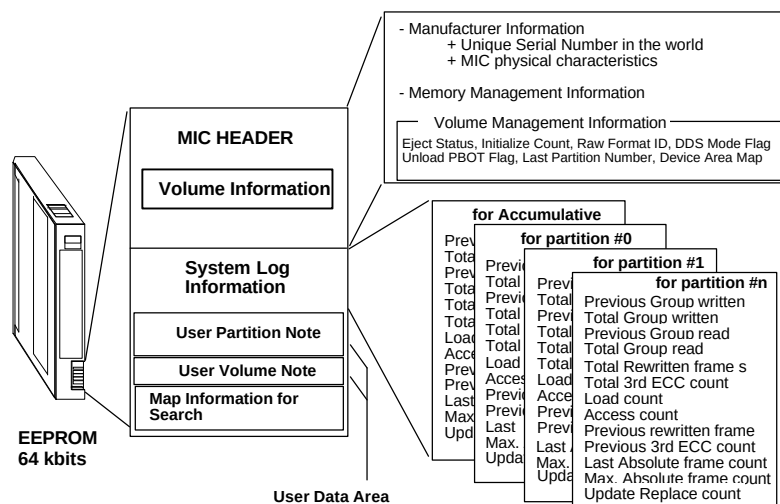
Figure E-2: MIC Data Structures
