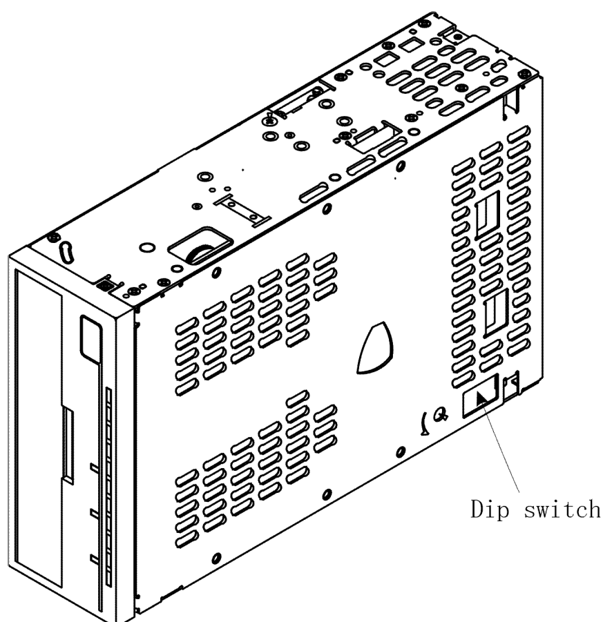
Figure 3-1: DIP switch
