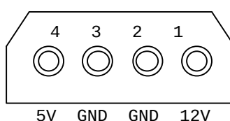
Figure 3-5: Power Connector
