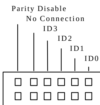
Figure 3-2: Jumper positions
