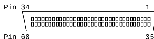
Figure 3-4: Non-shielded SCSI Device Connector
