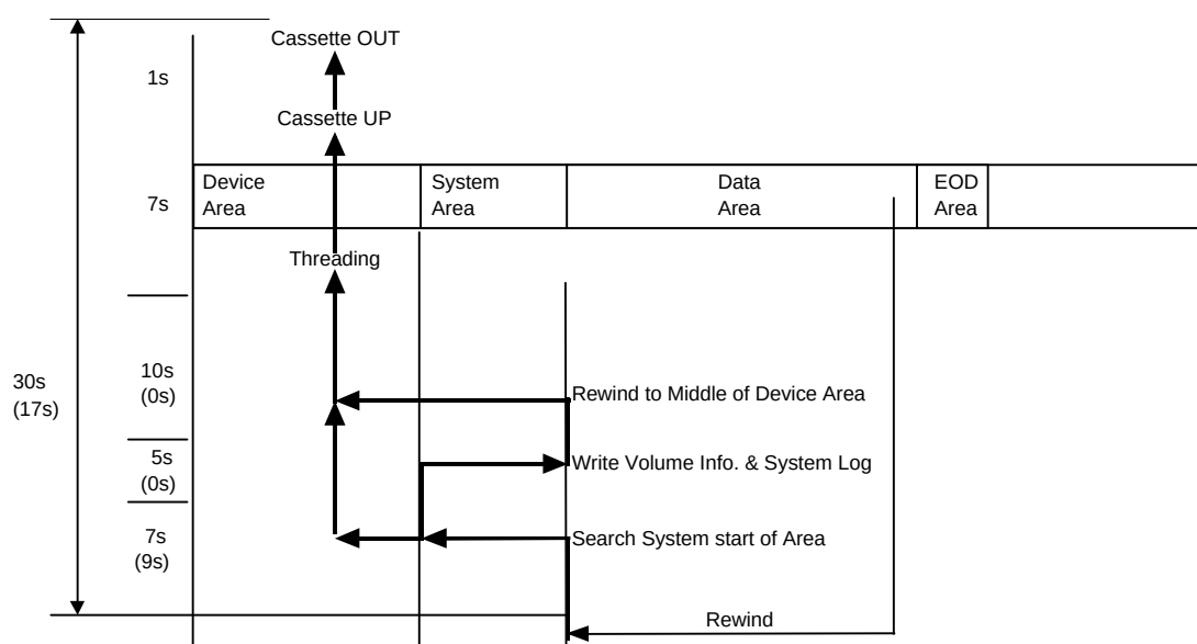
Figure E-4: Tape Unload with and without MIC
