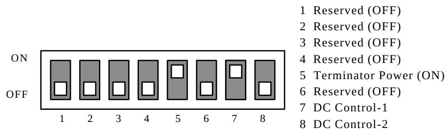
Figure 3-3: DIP Switch positions
