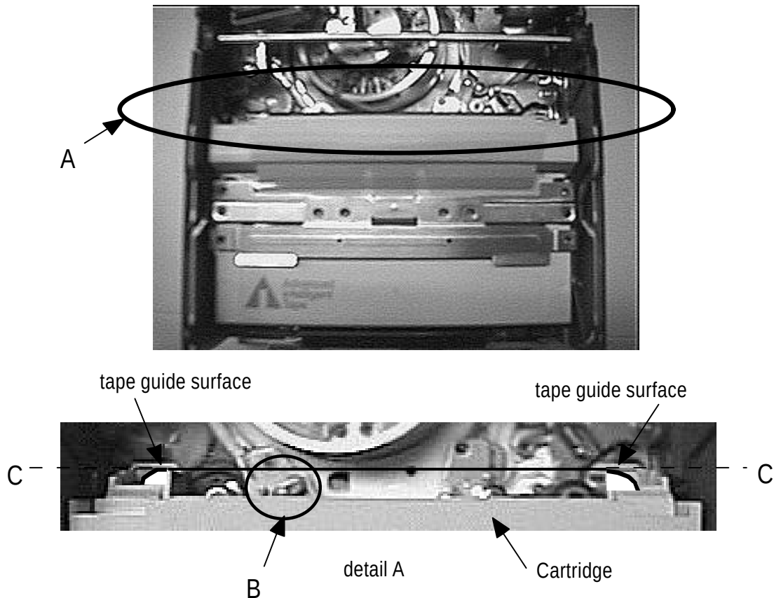
Photo 1: The Initial Position of the Threading Mechanism
