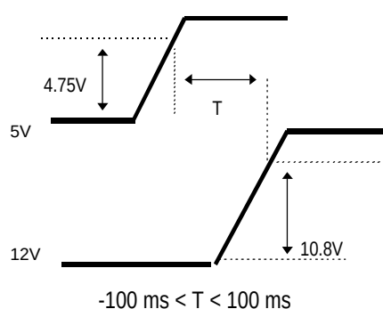
Figure 2-5: Power-up Sequence
