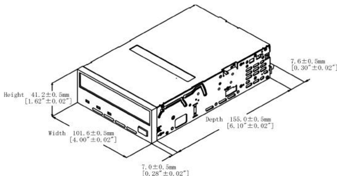
Figure 2-1: Dimensions (SDX-500C)
