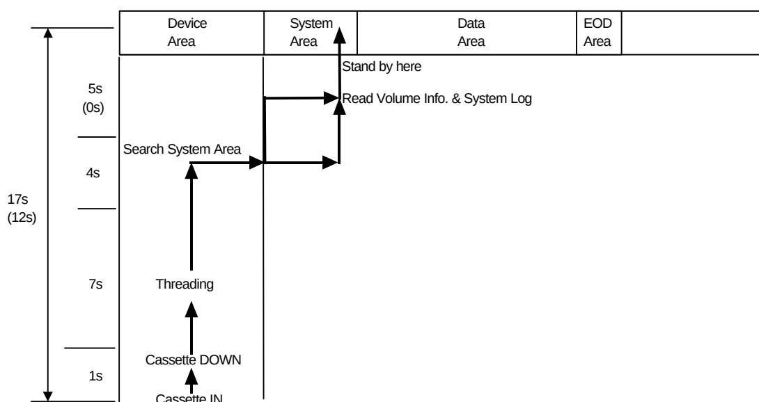
Figure E-5: Tape Load with and without MIC
