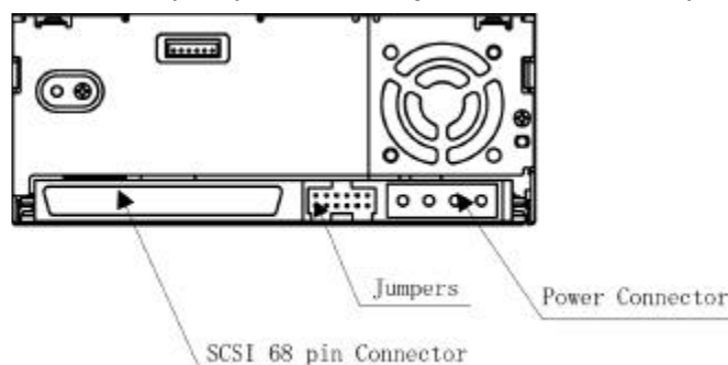
Figure 2-3: Connector Positions
